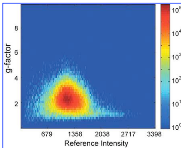
FIG. 6. Logarithmic histogram of g-factors computed for each voxel in the brain of the acquired volume. Median g-factor 2.49. Geometry factors tend toward unity with greater reference image intensity because of the method's dependence on phase.
